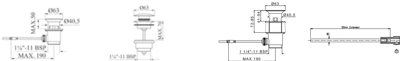
Automatic water waste for special furniture
