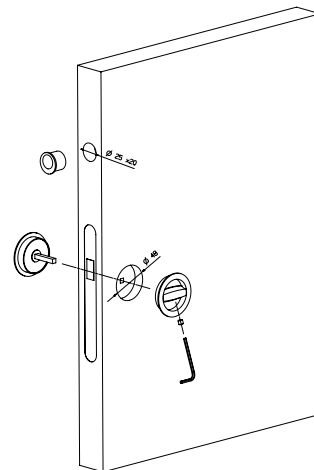
Montaggio kit incasso / Fitting of built-in kit
