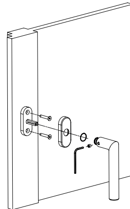
Montaggio maniglia per finestra DK 4-8-scatti / Handle fitting for tilt windows 4-8-clicks
