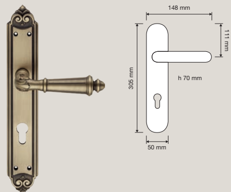
1611 PL Maniglia con placca Small / Door handle on plate Small
