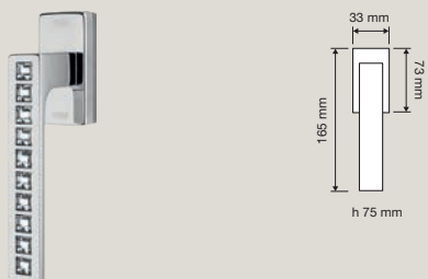
321 PB 0024 Pomolo per mobile / Cabinet knob
